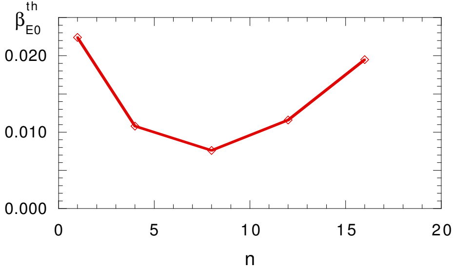
Figure 1: On axis value of the critical \beta_E , \beta_{E0}^{th} , for EPM excitation as n changes. Values as low as \beta_{E0}^{th} = 0.75\% are obtained for n = 8 EPM excitation with \rho_{LE}/a = 0.01 and a pressure profile, \beta_E = \beta_{E0} \exp(-r^2/L_{pE}^2) , with L_{pE}/R_0 \simeq 0.075 and a/R_0 = 0.1 [17].
