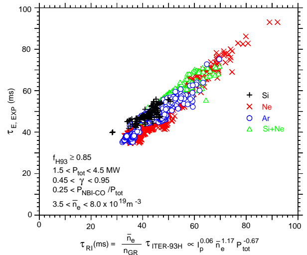
Figure 3. Comparison between the experimentally observed confinement times and the predictions of the RI-mode scaling law \tau_{RI} = (\bar{n}_e/n_{GR})\tau_{ITERH93-P} \propto I^{0.06} n_e^{1.17} P_{tot}^{-0.67} for Ne, Ar, Si and Si+Ne seeded RI-mode discharges in TEXTOR-94.
