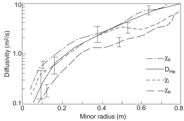
Figure 26. Similarity of the toroidal momentum diffusivity \chi_\phi , helium diffusion coefficient, D_{\text{He}} , and ion and electron thermal diffusivities, \chi_i and \chi_e , in a hot ion L-mode discharge in TFTR [379].
