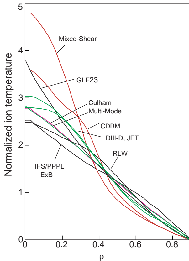
Figure 23. Normalized ion temperature profiles, [T_i(\rho) - T_i(0.9)] / \langle T_i(\rho) - T_i(0.9) \rangle , compared between various local transport models and for DIII-D and JET ITER demonstration discharges.
