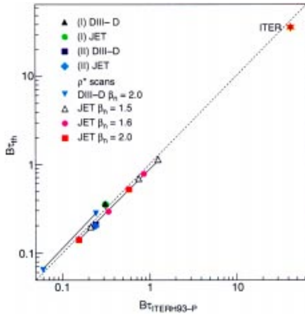
Figure 15. Comparison of B\tau_E measured in \rho^* scans on JET and DIII-D with the ITER93H-P scaling relation.
