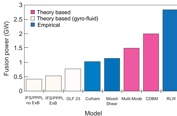
Figure 20. Fusion power predicted by various models with an edge temperature T(0.9) = 3 keV.
