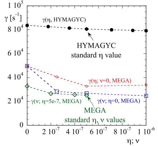
Figure 3. Growth-rate vs resistivity (HYMAGYC and MEGA) and vs viscosity (MEGA) for one of the reference cases considered in this paper (see section 4.1, peaked-on axis EP radial density profile).
