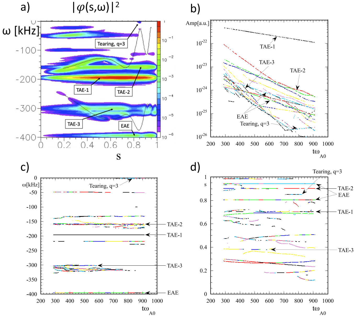
Figure 7. Frequency power spectra of the e.s. field |\varphi(s, \omega)|^2 for the HYMAGYC simulation shown in figure 6 (only negative portion of the frequency plane), with the identification of the dominant modes observed (a). Amplitude (b), frequency (c), and radial position (d) versus time of the relative maxima of the frequency spectra of the HYMAGYC simulation shown in (a). A fixed sequence of colors (related to the values of the \text{amp}_{\text{rel. max.}}(t) : black the highest value, red the second highest, and then green, blue, yellow, violet and cyan, and then cycled) is used for each time; the same colors of the dots are used also for the other plots (c) and (d), to help the identification of the modes.
