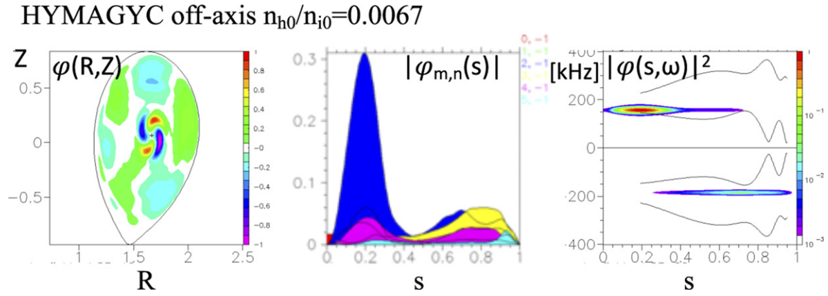
Figure 13. HYMAGYC: peaked off-axis EP density profile, with n_{h0}/n_{i0} = 0.0067 : e.s. field structure \varphi(R, Z) in the poloidal plane \phi = 0 (left), radial profiles of the Fourier components |\varphi_{m,n}(s)| (centre), and frequency power spectra |\varphi(s, \omega)|^2 (right). The dominant core localized TAE ( s \lesssim 0.4 ), with preeminent m = 2 poloidal Fourier component is observed in the central region, with a positive real frequency; in the external region ( s \gtrsim 0.4 ) it is also present the sub-dominant external TAE, with a preeminent m = 3 poloidal Fourier component and a negative real frequency (i.e. with opposite sign w.r.t. the dominant internal mode).
