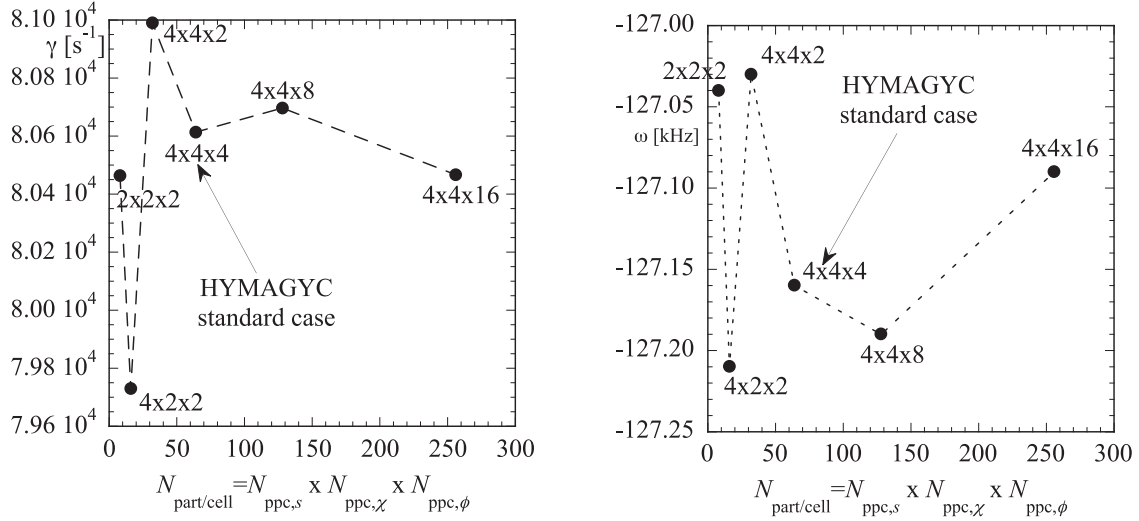
Figure 4. Growth-rate (left) and frequency (right) vs the number of EPs per cell, N_{\text{part/cell}} obtained by HYMAGYC for one of the reference cases considered in this paper (see Sec. 4.1, peaked-on axis EP radial density profile).
