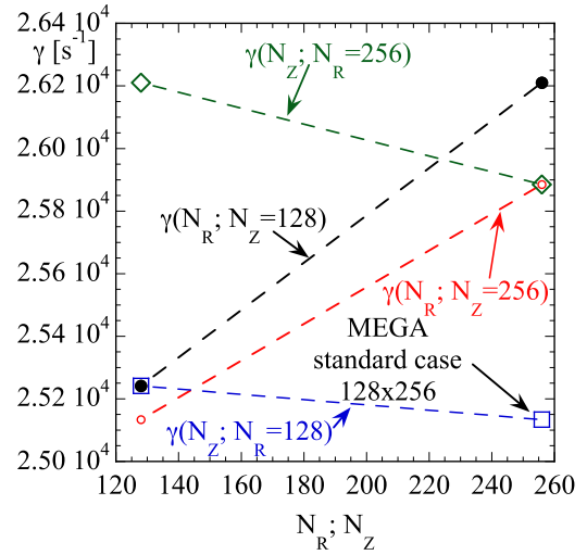
Figure 5. Growth-rate vs the number of grid points N_R or N_Z obtained by MEGA for one of the reference cases considered in this paper (see section 4.1, peaked-on axis EP radial density profile).
