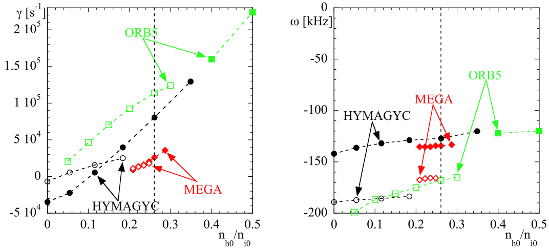
Figure 10. EP density scan for the AUG on-axis EP density profile: growth rates (left frame) and frequencies (right frame). Black circles refer to HYMAGYC results, red diamonds to MEGA, and green squares to ORB5, with closed symbols indicating RSAEs and open symbols to TAEs. The dashed black vertical lines refer to the nominal value of n_{h0}/n_{i0} .
