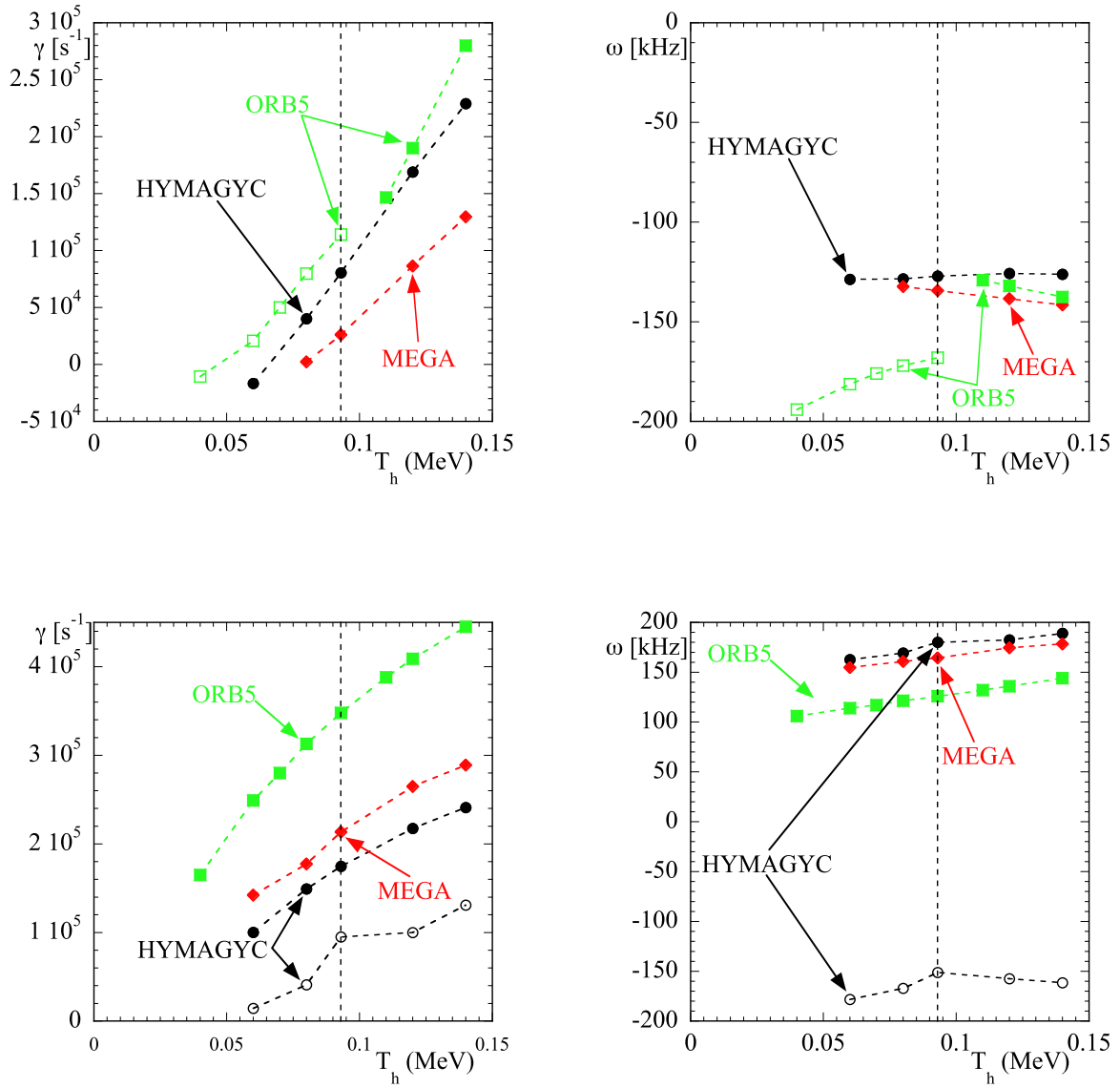
Figure 14. Growth rates (left column) and frequencies (right column) vs T_h for the on-axis (top row) and off-axis (bottom row) EP density profiles. Black circles refer to HYMAGYC results, red diamonds to MEGA, and green squares to ORB5. The dashed black vertical lines refer to the nominal value of T_{h0} .
