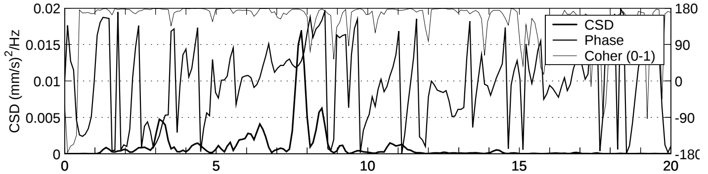
c170512 CSD/COHER 5-6
