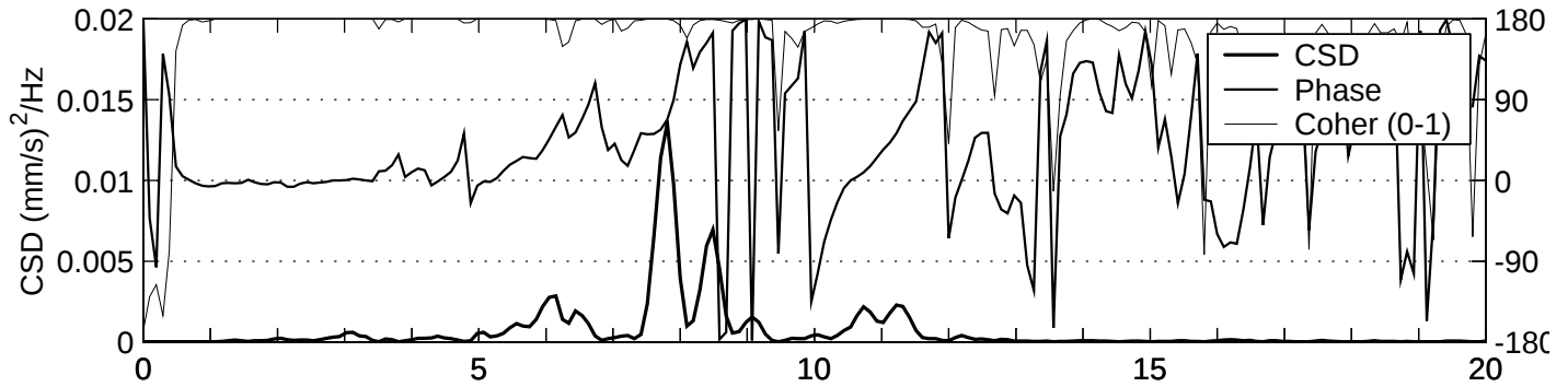
c170512 CSD/COHER 4-6
