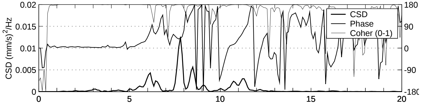
c170512 CSD/COHER 2-5
