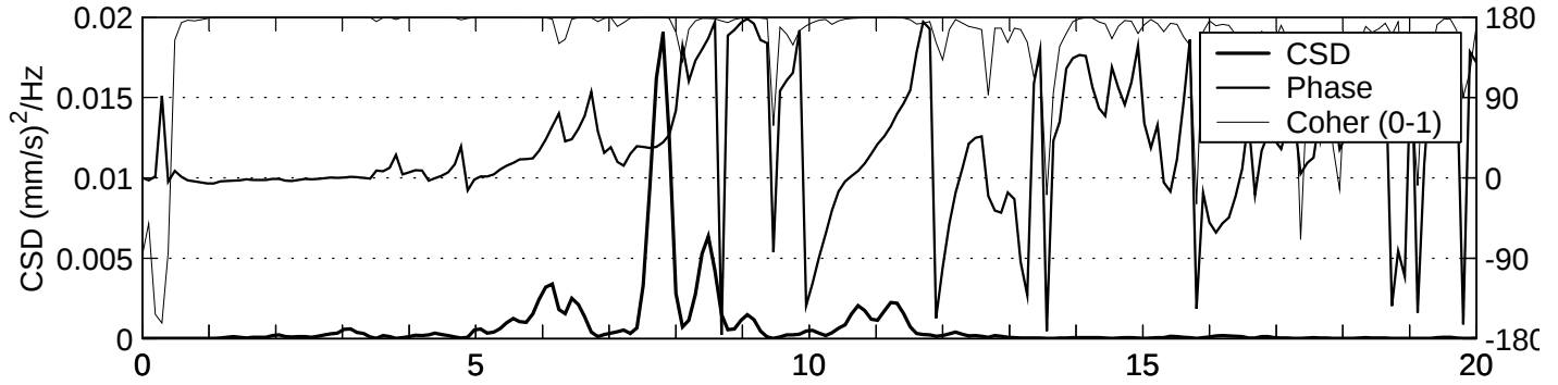
c170512 CSD/COHER 2-6
