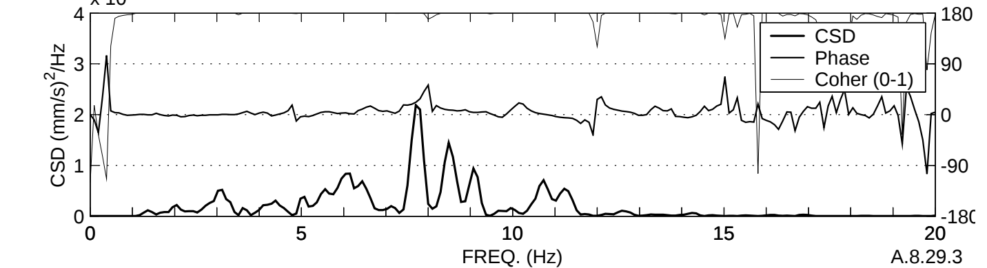
c170512 CSD/COHER 5-6
