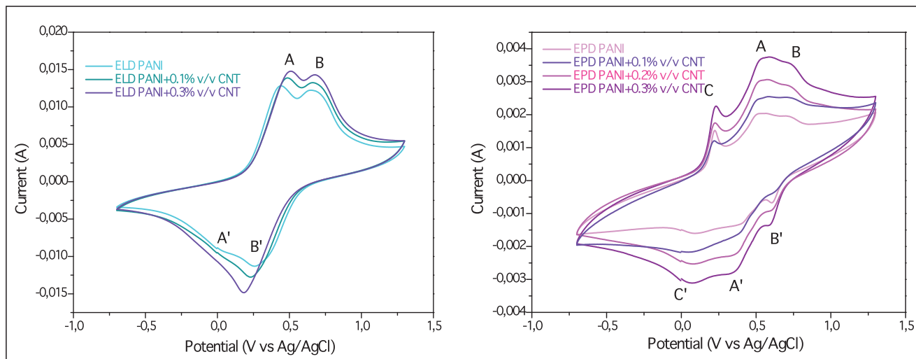
FIGURE 8 CV in \text{H}_2\text{SO}_4 of ELD PANI-CNTs (a) and EPD PANI-CNTs (b) (the CV referring to 0.2% v/v CNT of ELD composites was omitted for better clarity of the graph)
