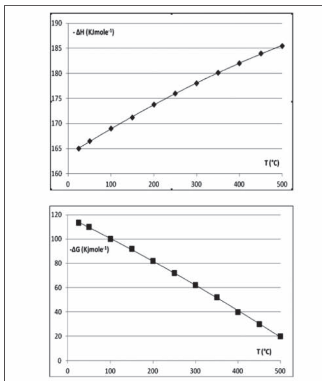
FIGURE 1 Molar enthalpy and molar Gibbs free energy for Sabatier reaction in the temperature range 25 °C - 500 °C Source: ENEA
