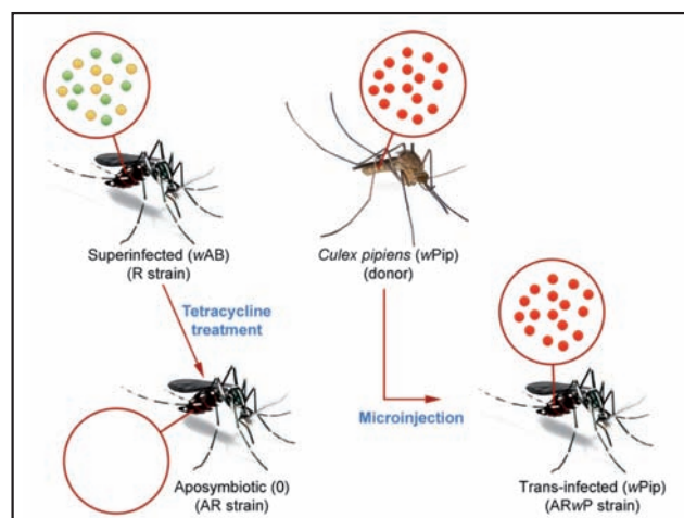
FIGURE 3 Outline of the protocol to generate a new Wolbachia infection in Ae. Albopictus . Isolines of mosquitoes Wolbachia -free are generated via antibiotic treatment of superinfected wild mosquitoes. Wolbachia drawn from Culex pipiens embryos is then microinjected into embryos of the Wolbachia -free Ae. albopictus line.
