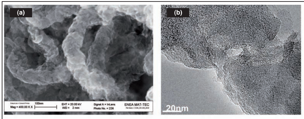
FIGURE 4 CNF with turbostratic structure: SEM (a) and High Resolution TEM (b) images
