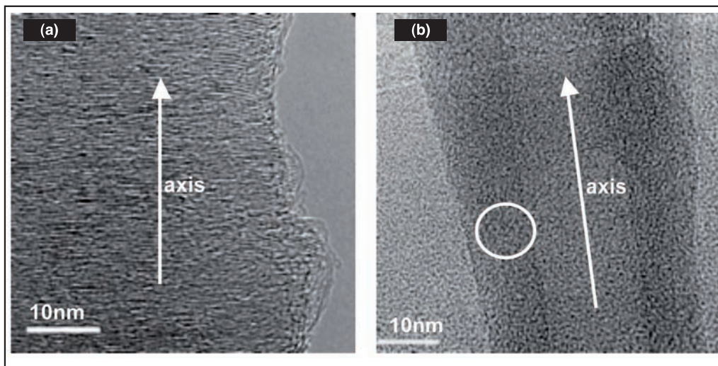
FIGURE 3 TEM images showing the structure of platelet (a) and tubular (b) CNFs
