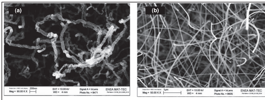
FIGURE 2 FEG-SEM micrograph of platelet (a) and tubular (b) CNFs
