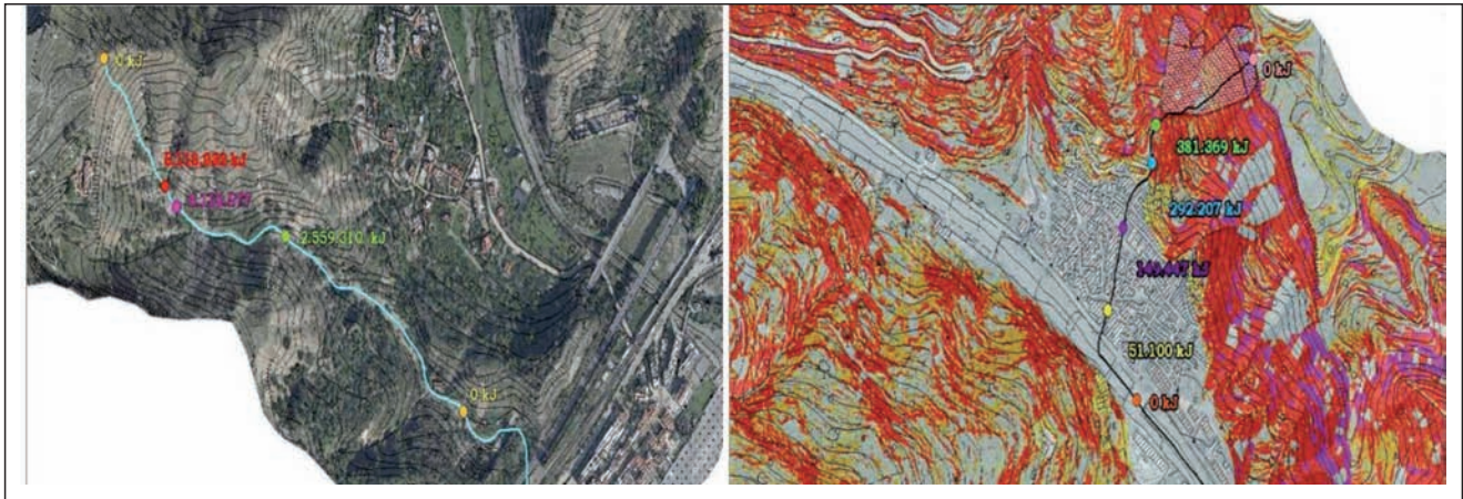
FIGURE 6 Maximum developed energies in the Fallega creeks between Giampilieri Marina (a) and Briga Marina and maximum energies of the potential debris flow in the Giampilieri village (b)
