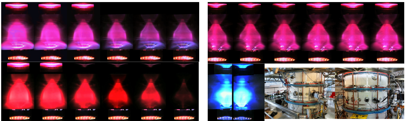
Left: Switch-off of H-Torus - top visible light, bottom H \alpha light
