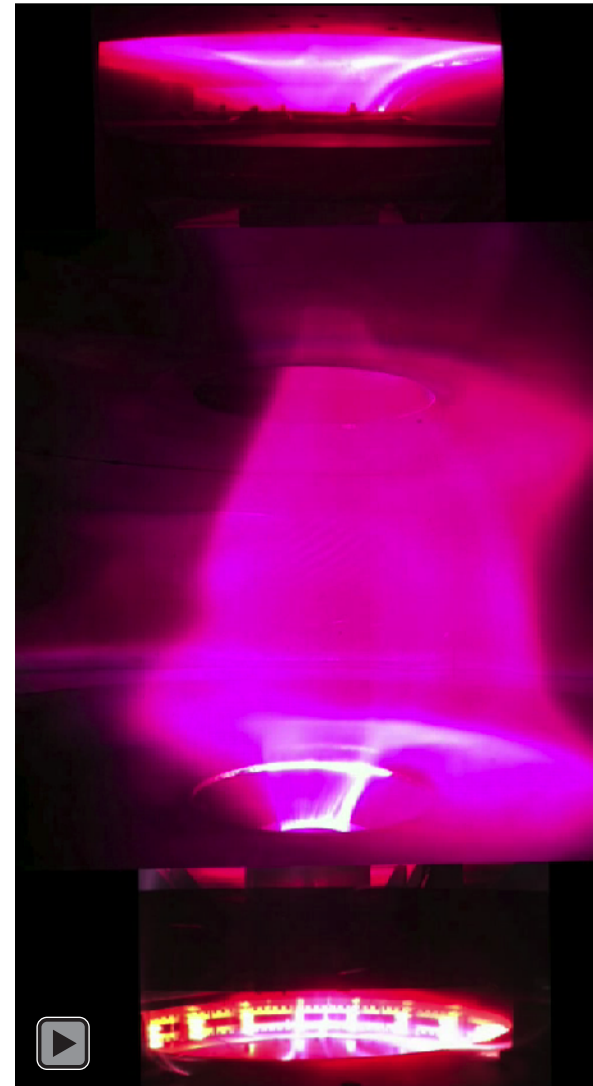
#1225 Hydrogen
