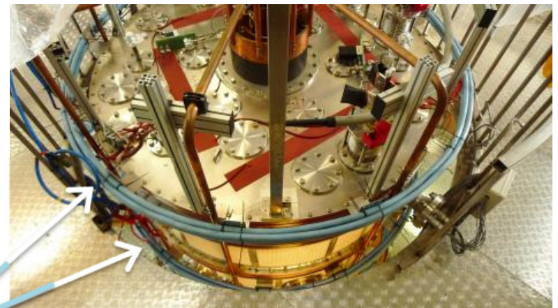
4 external PF coils
