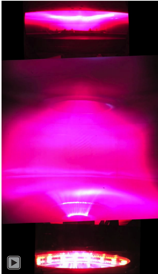
#1211 Hydrogen
