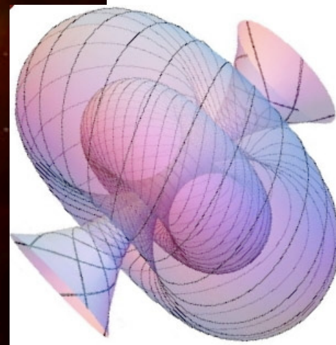
Hopf foliation
