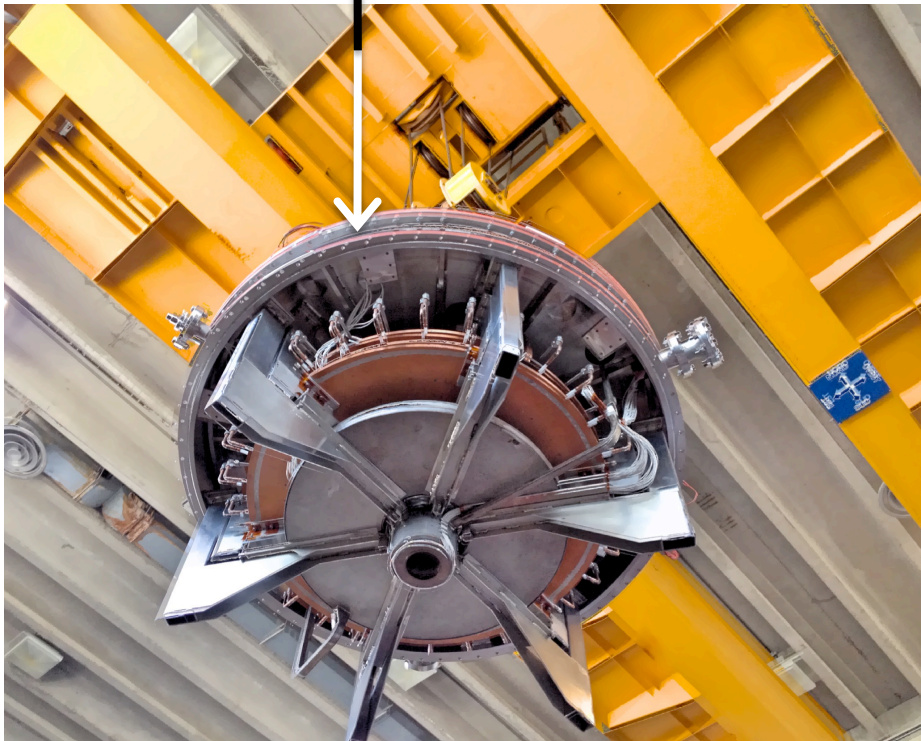
Assembly of the annular anode on the machine (May 2015)
