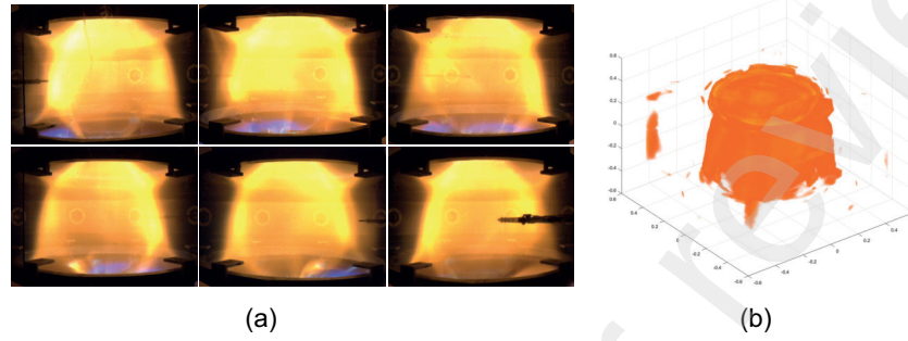
Figure 10: a) Pictures recorded by the six cameras at a given time instant (267 msec) of the PROTO-SPHERA experiment from shot 2505 of Helium b) 3D reconstruction of plasma light emission density
