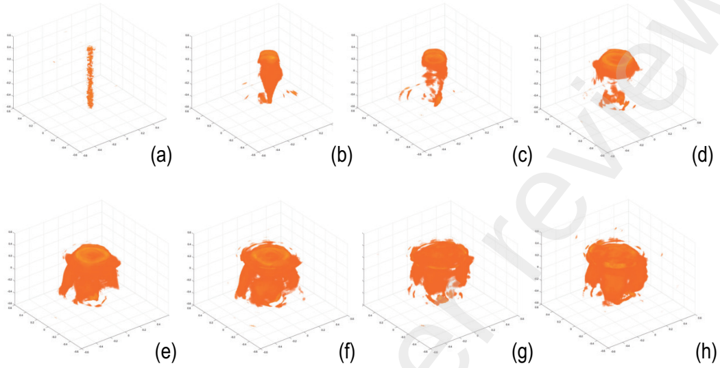
Figure 12: Reconstructed light emission density of Helium discharge 2505 at eight sequential time steps: stable pinch (a-b), pinch instability (c-f), formation of the plasma torus around the pinch (g-h)
