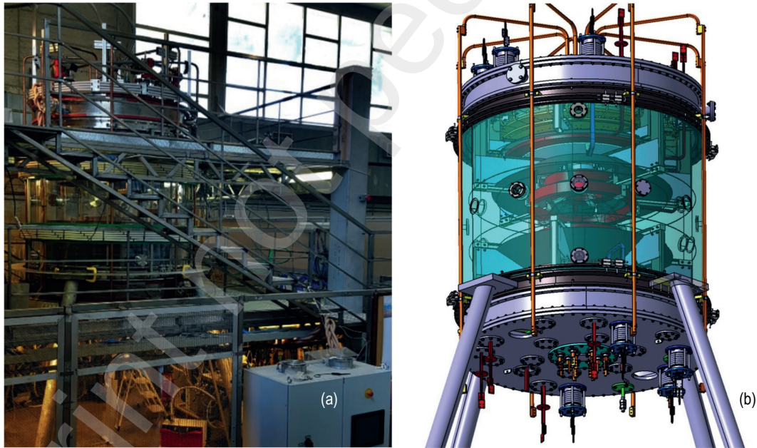
Figure 8: Picture of PROTO-SPHERA setup and schematic of the machine b)
