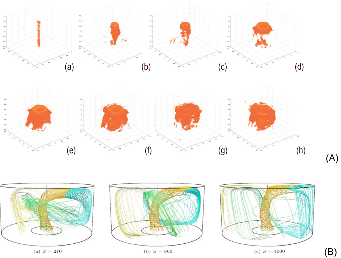
Figure 3: Comparison of Figure 12 of the submitted manuscript (A) with Figure 9 (B) of the paper by Garcia-Martinez et al., which represents the field lines of the magnetic field at different Lundquist numbers.
