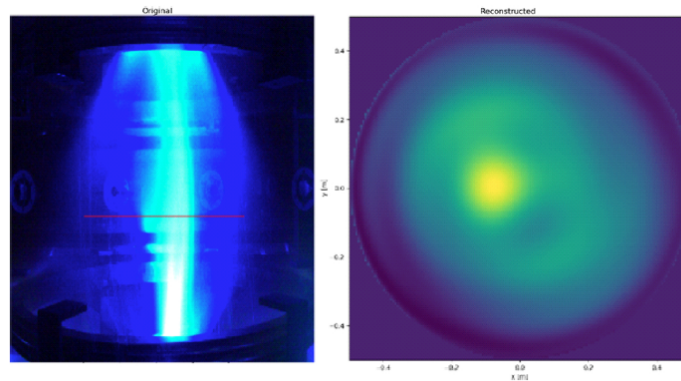
Figure 5: Pictures and related equatorial distribution of Argon plasma luminosity obtained by Zernicke polynomials inversion (Y. Damizia et al. Optical tomography of the plasma on the PROTO-SPHERA experiment (2021))
