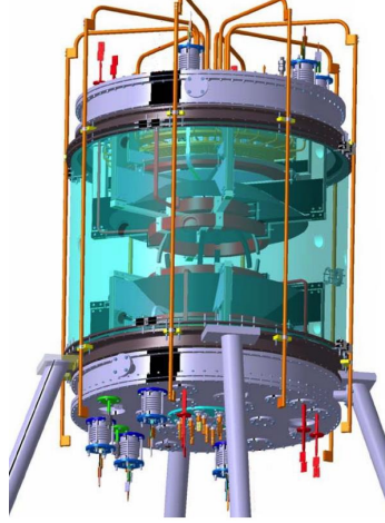
Figure 8: Schematic of the PROTO-SPHERA experiment
