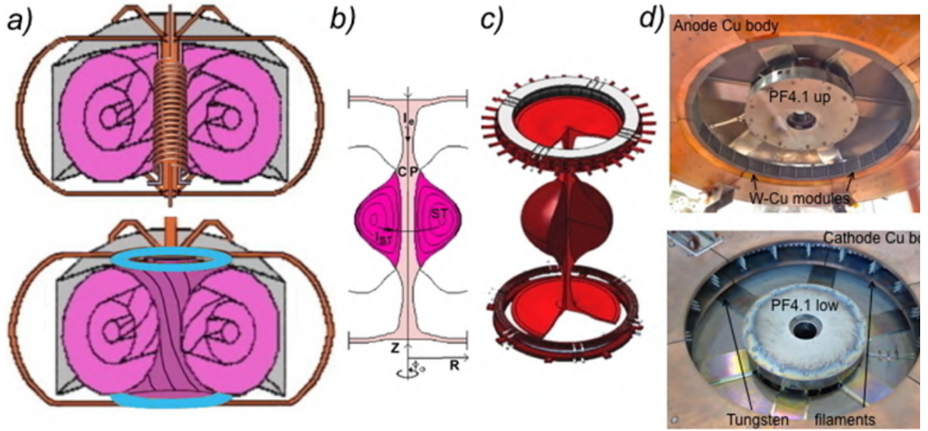
Figure 1. (a) Scheme of a Tokamak (top) and of PROTO-SPHERA (bottom): pink colour is for plasma, grey for vessel, orange for metal bars, blue for electrodes. (b) Poloidal cross-section of PROTO-SPHERA plasma, CP stands for centerpost, ST for torus, the mechanical structures of the poloidal field coils are removed from the scheme. (c) Perspective sketch of the plasma and of the annular electrodes. (d) View of the annular anode (top) and of the annular cathode (bottom).
