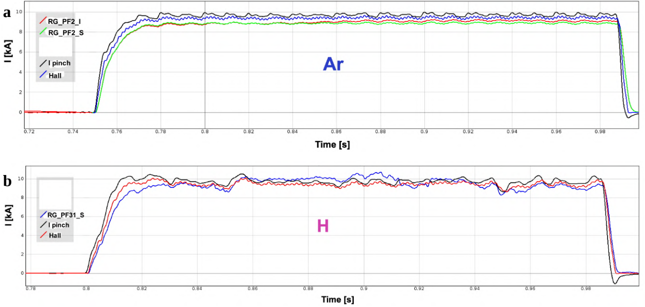
Figure 12. (a) Argon discharge #1037 at I_{\text{CP}}=10 kA: waveforms of I_{\text{CP}} the plasma centerpost current as measured on the power supply and on the return bars of the machine (by Hall sensors) compared with the traces of two in-vessel Rogowski sensors. (b) Hydrogen discharge #1010 at I_{\text{CP}}=10 kA: waveforms of the plasma centerpost current as measured on the power supply and on the return bars of the machine (by Hall sensors) compared with the trace of one in-vessel Rogowski sensor.
