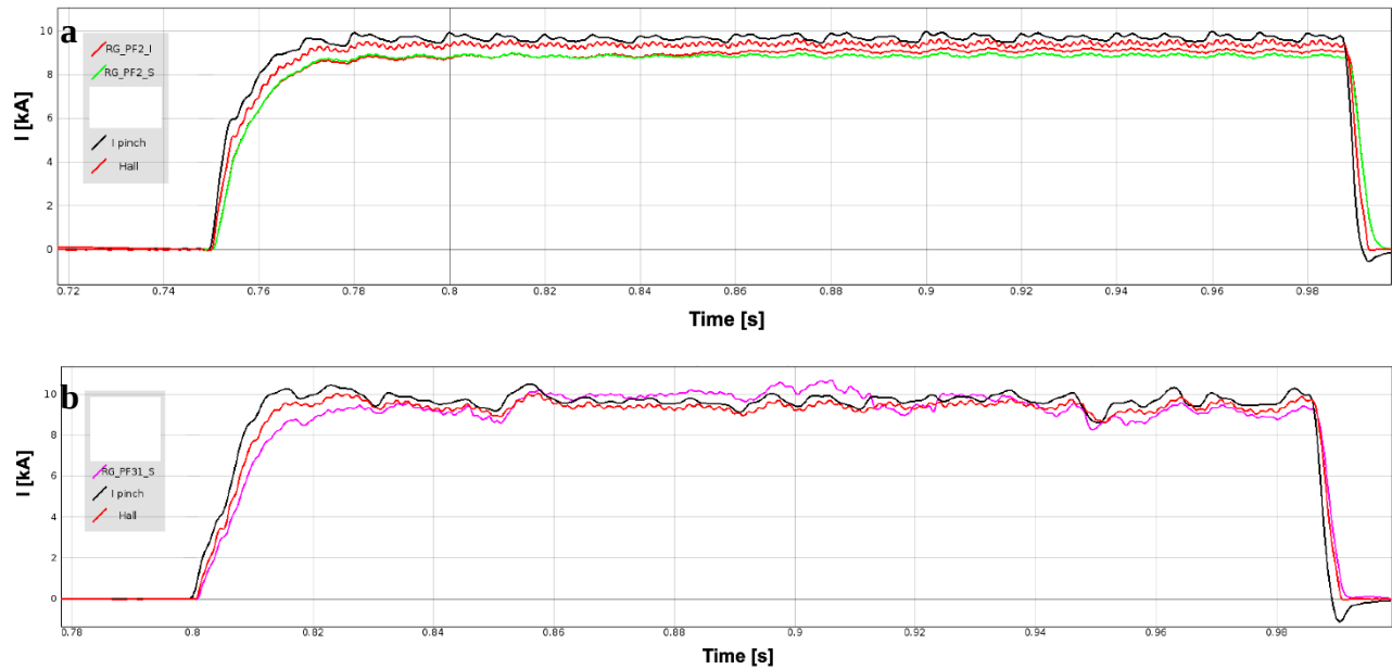
Figure 12. (a) Argon discharge #1037 at I_e = 10 kA: waveforms of I_{\text{CP}} the plasma centerpost current as measured on the power supply and on the return bars of the machine (by Hall sensors) compared with the traces of two in-vessel Rogowski sensors. (b) Hydrogen discharge #1010 at I_e = 10 kA: waveforms of the plasma centerpost current as measured on the power supply and on the return bars of the machine (by Hall sensors) compared with the trace of one in-vessel Rogowski sensor.
