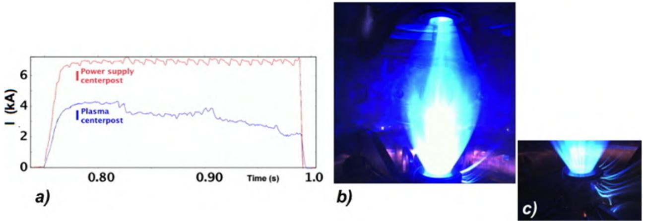
Figure 9. (a) Waveforms of Argon centerpost plasma current, evidencing a slow decrease of plasma centerpost current I_e . (b) and (c) Spurious plasma currents with filamentary patterns near the lower PF2 mirror coil. All figures refer to shot #597.
