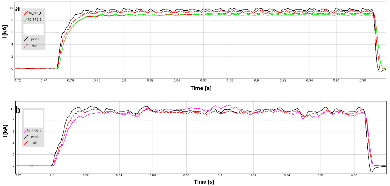
Figure 12. (a) Argon discharge #1037 at I_e=10 kA: waveforms of I_{\text{CP}} the plasma centerpost current as measured on the power supply and on the return bars of the machine (by Hall sensors) compared with the traces of two in-vessel Rogowski sensors. (b) Hydrogen discharge #1010 at I_e=10 kA: waveforms of the plasma centerpost current as measured on the power supply and on the return bars of the machine (by Hall sensors) compared with the trace of one in-vessel Rogowski sensor.
