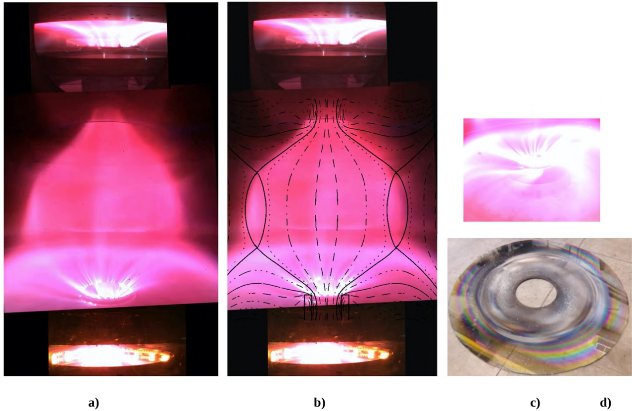
Figure 14. (a) "Lean" torus visible as a brighter belt at the outer edge of the Hydrogen plasma centerpost. (b) Same, with superposed equilibrium calculation of magnetic flux surfaces. (c) Lower magnetic separatrix, just below the lower circle of X points, from a different camera. All three images refer to Hydrogen plasma shot #1280. (d) Polycarbonate lower diaphragm, removed at the end of the experimental campaign in which PROTO-SPHERA produced the first plasma tori.
