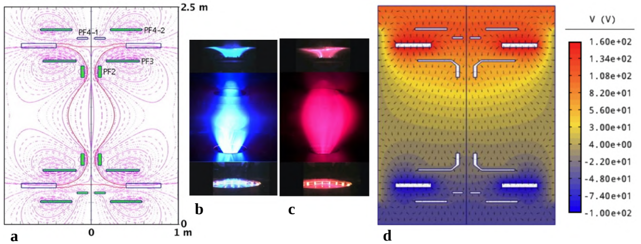
Figure 11. (a) Shaping magnetic field, up/down symmetric, produced by the eight Group-B-PFInt coils, the four upper coils are denominated in this figures, the lower four ones being mirror symmetric across the equatorial plane. (b) Argon centerpost discharge #1037 at I_{CP}=10 kA: pictures from 3 cameras (at different azimuthal angles) are superposed. (c) Hydrogen discharge #1010 at I_{CP}=10 kA. (d) The electrostatic potential in H discharges at I_{CP}=10 kA (shown with different colors) is not up/down antisymmetric, i.e. the plasma charges the Group-B-PFInt coils on the anode side with a different pattern of electric potential with respect to the cathode side.
