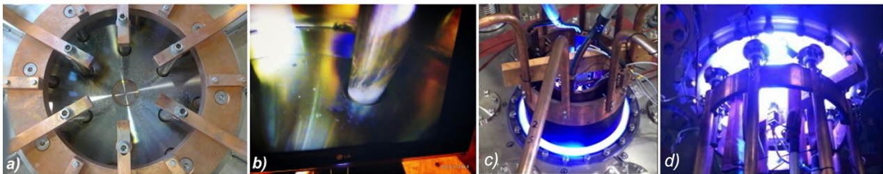
Figure 4. In presence of AISI304 central lid flanges: (a) Anode top busbars viewed from inside the vessel. (b) Enlarged view of one of the cathode bottom busbar, also from the inside, showing a relevant metallization. (c) The visible light of an Argon plasma centerpost emerging from the upper anodic polycarbonate flange, shot #567. (d) The visible light of an Argon plasma centerpost emerging from the lower cathodic polycarbonate flange, shot #577.
