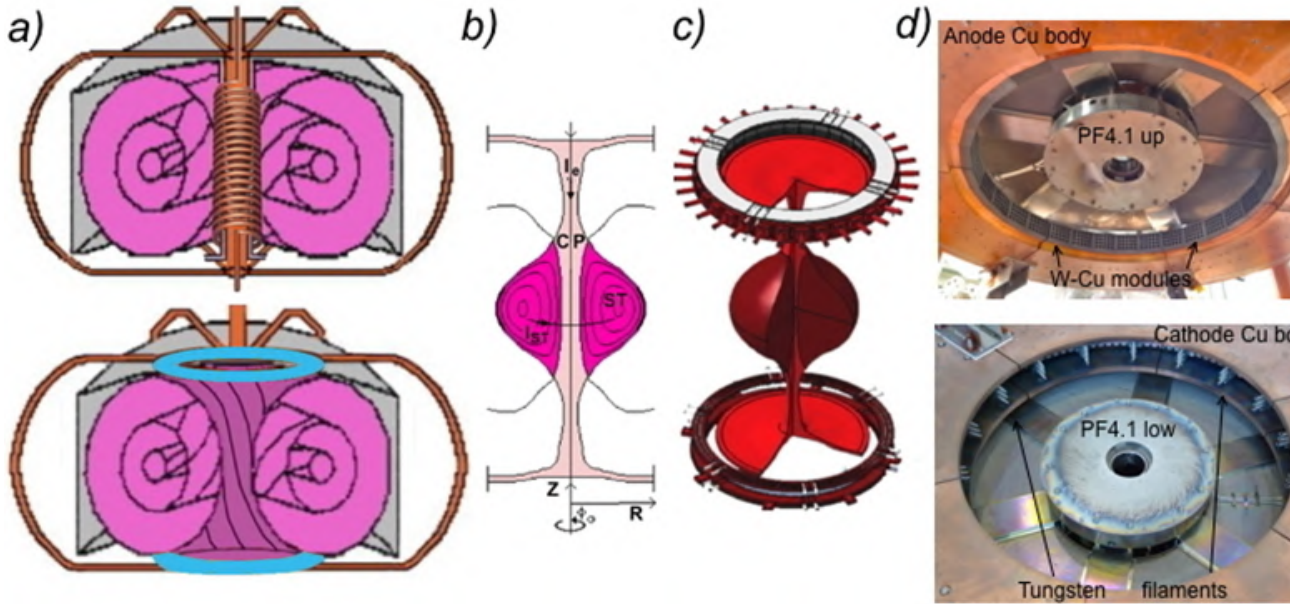
Figure 1. (a) Scheme of a Tokamak (top) and of PROTO-SPHERA (bottom): pink colour is for plasma, gray for vessel, orange for metal bars, blue for electrodes. (b) Poloidal cross-section of PROTO-SPHERA plasma, CP stands for centerpost, ST for torus, the mechanical structures of the poloidal field coils are removed from the scheme. (c) Perspective sketch of the plasma and of the annular electrodes. (d) View of the annular anode (top) and of the annular cathode (bottom).
