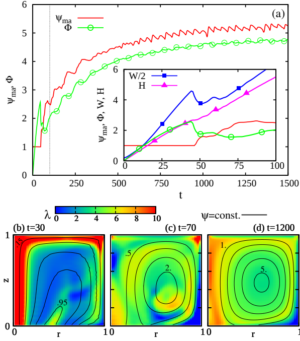
FIG. 1: (Color online) Evolution of \psi_{ma} and \Phi (a). In the inset, the evolution for t < 100 is showed in more detail. In addition the (halved) magnetic energy and the helicity are shown. Colormaps of \lambda and \psi contours in the poloidal plane are shown at three different times (b)-(d).
