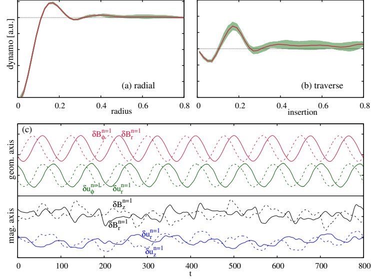
FIG. 15: (Color online) (a) Radial and (b) traverse E_{dyn} profiles obtained at the locations indicated with white lines in Fig. 14 (b.1). (c) Temporal signals of the perpendicular n = 1 fluctuations of velocity and magnetic field at the geometric and magnetic axis.
