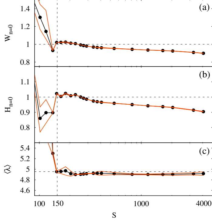
FIG. 5: (Color online) (a) Magnetic energy, (b) relative magnetic helicity of the n = 0 mode and (c) \langle \lambda \rangle = 2W_{n=0}/H_{n=0} during steady state. The energy and helicity are normalized to their initial values. Average values, during the sustainment phase, are shown with black lines and points while the maximum and minimum values are shown with orange lines.
