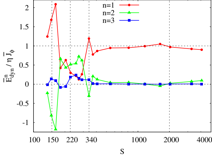
FIG. 16: (Color online) Average dynamo electric field at the magnetic axis of the first three toroidal modes.
