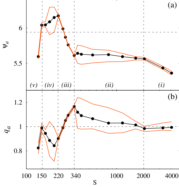
FIG. 6: (Color online) Poloidal flux (a) and safety factor (b) at the magnetic axis during the sustainment phase. Maximum and minimum values are in orange and the average is in black.
