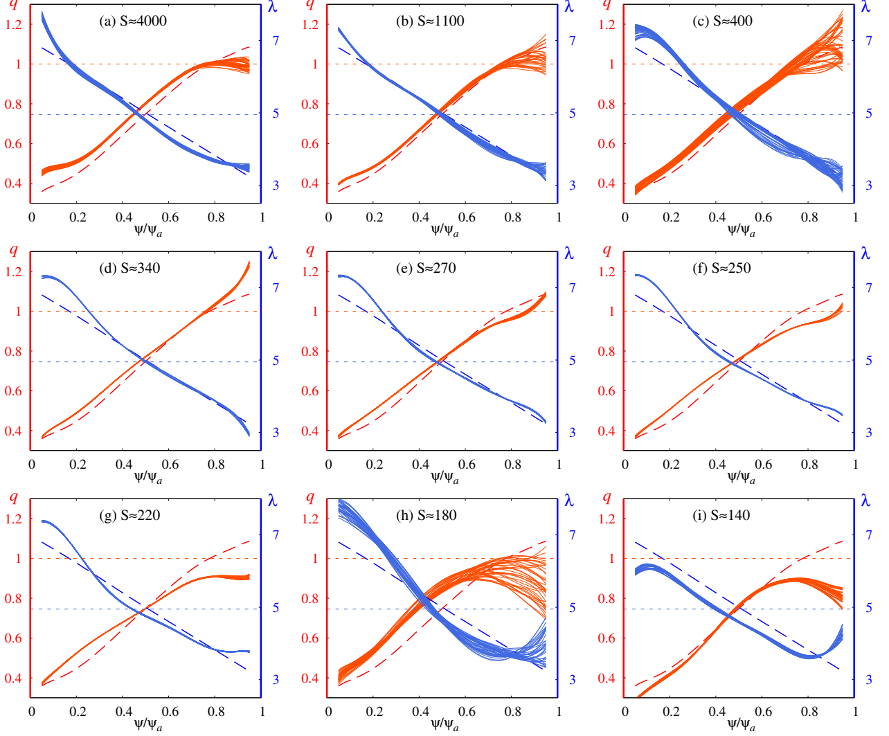
FIG. 7: (Color online) q and \lambda profiles during sustainment. Fifty instantaneous profiles during the sustainment phase are shown for each variable. The initial profiles are shown with dashed lines.
