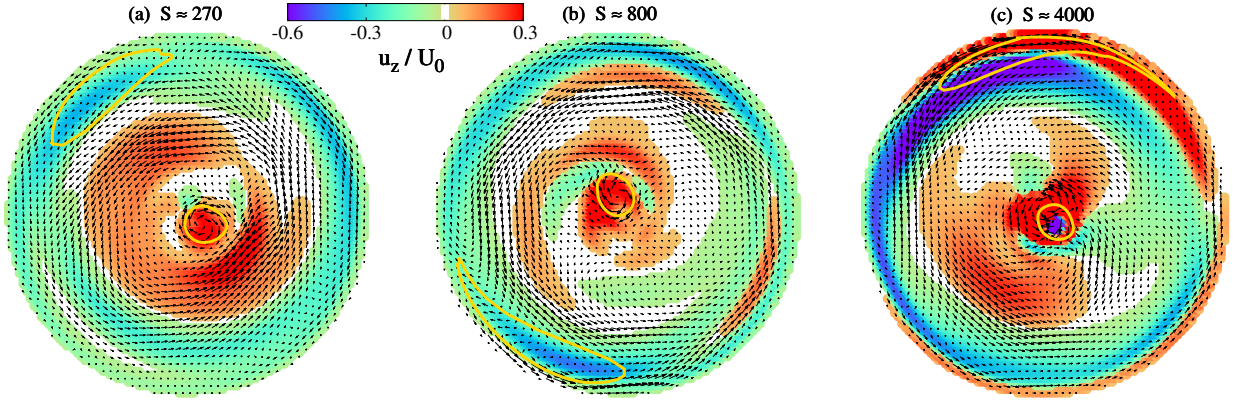
FIG. 12: (Color online) Mean flow during sustainment. The colormaps indicate the toroidal flow and the arrows the poloidal flow. The flow is normalized with the corresponding U_0 value in each case.
