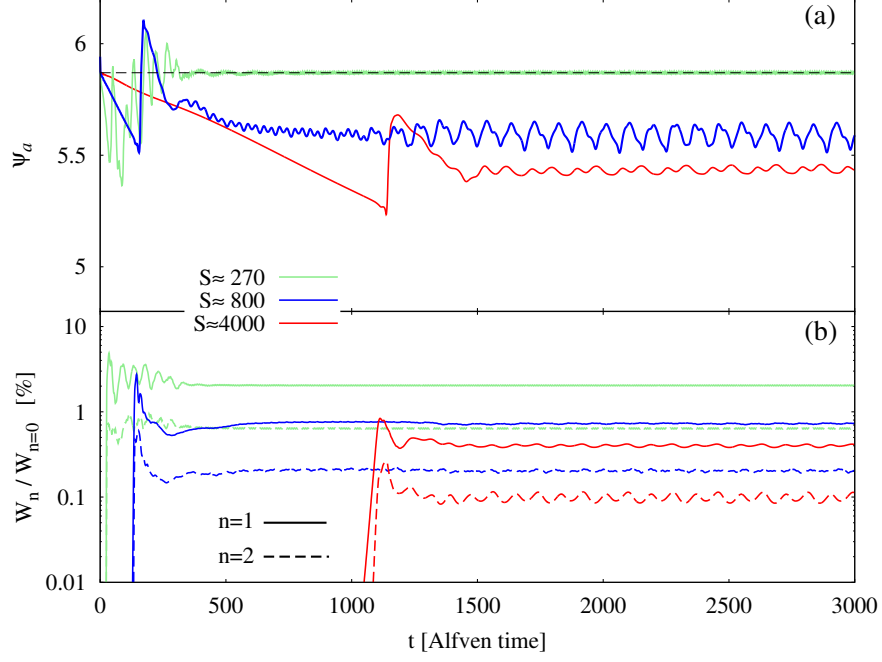
FIG. 3: (Color online) (a) Evolution of the poloidal flux at the magnetic axis and (b) the magnetic energy content of the first two toroidal modes (relative to the n = 0 magnetic energy) for three cases.
