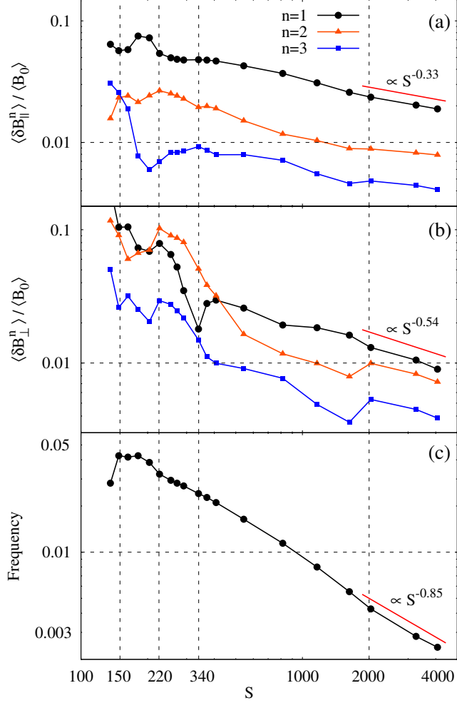
FIG. 11: (Color online) Mean fluctuation level, relative to the mean field, of the three dominant modes during sustainment at the magnetic axis as a function of S : (a) parallel and (b) perpendicular components. (c) The frequency of the parallel fluctuation, normalized with the Alfvén time, is also shown.
