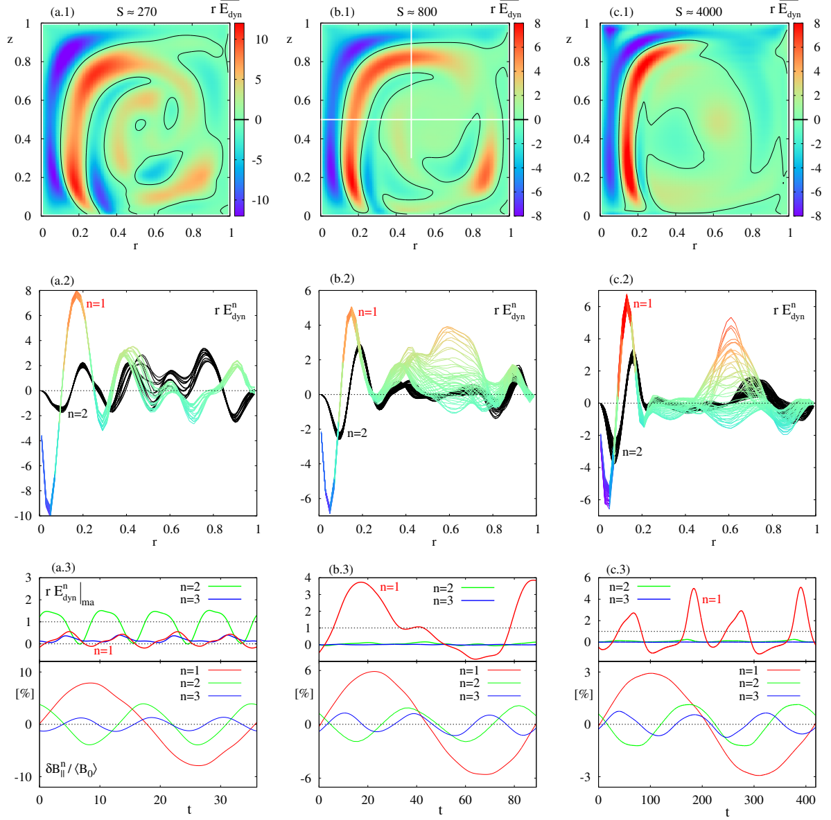
FIG. 14: (Color online) Colormaps of the mean (in time) total dynamo electric field multiplied by the radial coordinate (a.1) - (c.1). The black line is the contour r \bar{E}_{dyn} = 0 . Several radial profiles of the instantaneous value of r E_{dyn}^n for n = 1 and n = 2 , at z = 0.5 (a.2) - (c.2). The colorscale of the n = 1 profiles is the same than that of the corresponding colormap. Evolution of r E_{dyn}^n at the magnetic axis and the relative parallel magnetic fluctuation for n = 1, 2 and 3 (a.3) - (c.3). All values are normalized with (r \eta \bar{J}_\theta)_{ma} .
