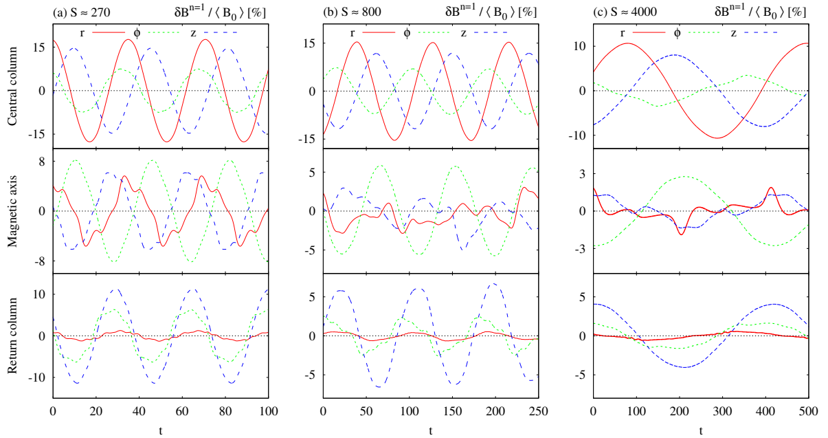
FIG. 10: (Color online) Evolution of the relative magnetic fluctuations of the n = 1 mode in three spatial locations: near the axis of symmetry (central column), at the magnetic axis and near the wall (return column). All values are taken at z = 0.5 . The three components of the magnetic field vector are displayed for three cases.
