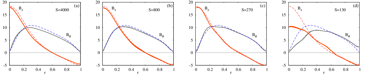
FIG. 4: (Color online) Poloidal ( B_z ) and toroidal ( B_\phi ) radial profiles at z = 0.5 of the n = 0 component. Fifty instantaneous profiles in the time interval 2000 \leq t \leq 3000 are plotted (full lines). The dashed lines show the initial profiles.
