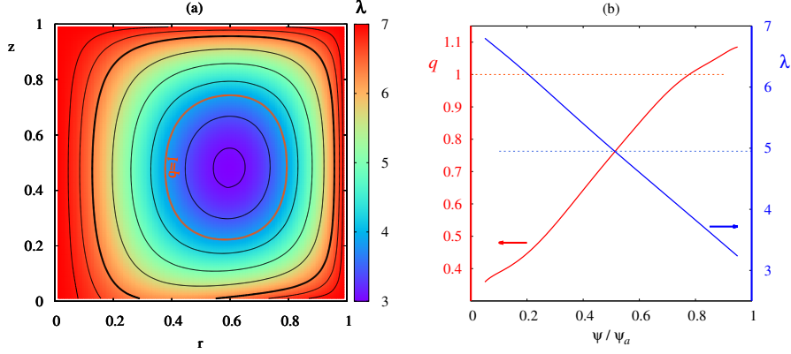
FIG. 2: Initial condition: (a) poloidal flux contours and colormap of \lambda and (b) profiles of \lambda and safety factor.
