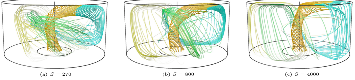
FIG. 9: (Color online) Field lines entering through the central electrode form a helical column that rotates almost rigidly. The prolongation of the central flux tube is strongly affected by the Lundquist number. (Enhanced online).
