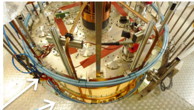
4 additional external PF coils
