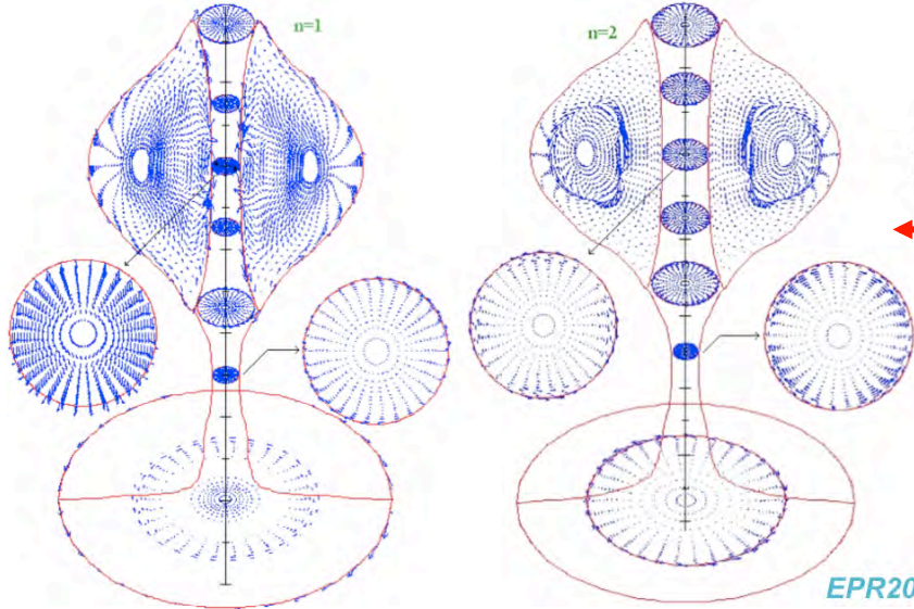
Examples of n=1 & 2 instabilities at high \beta
