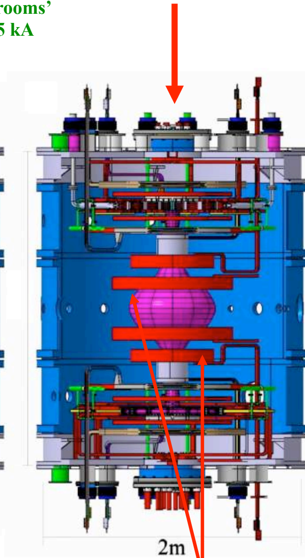
8 + 10 PF coils
