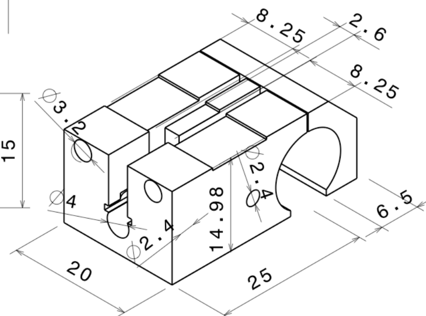
Isometric view Scale: 2:1
