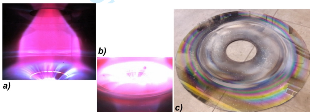
FIGURE 13. (a) "Lean" torus visible as a brighter belt at the outer edge of the Hydrogen plasma centerpost. (b) Lower magnetic separatrix, just below the lower circle of X points, from a different camera. Both from shot #1202. (c) Polycarbonate lower diaphragm, removed at the end of the experimental campaign in which PROTO-SPHERA produced the first plasma tori.
