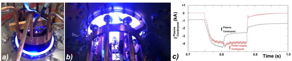
FIGURE 6. (a) The visible light of an Argon plasma centerpost emerging from the upper anodic polycarbonate flange, shot #567. (b) The visible light of an Argon plasma centerpost emerging from the lower cathodic polycarbonate flange, shot #577. (c) Waveforms of Argon centerpost plasma current, evidencing a sudden decrease after the centerpost discharge becomes attached to the Aluminium cylindrical vacuum vessel, shot #208.
