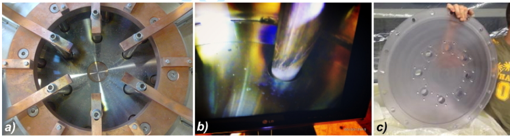
FIGURE 4. In presence of AISI304 central lid flanges: (a) Anode top busbars viewed from inside the vessel; (b) enlarged view of one of the cathode bottom busbar, also from the inside, showing a relevant metallization. (c) Large new anodic polycarbonate top lid flange.
