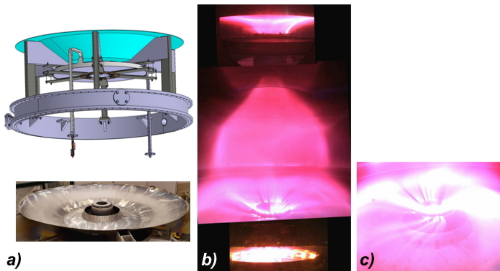
FIGURE 14. (a) CAD design of conical lower divertor plate (green-blue on top) and the first 0.5 mm thick AISI304 provisional lower divertor plate (bottom). (b) "Lean" torus visible as a brighter belt at the outer edge of the Hydrogen plasma centerpost, shot #1280. (c) Lower magnetic separatrix, just below the lower circle of X points, from a different camera, same shot.
