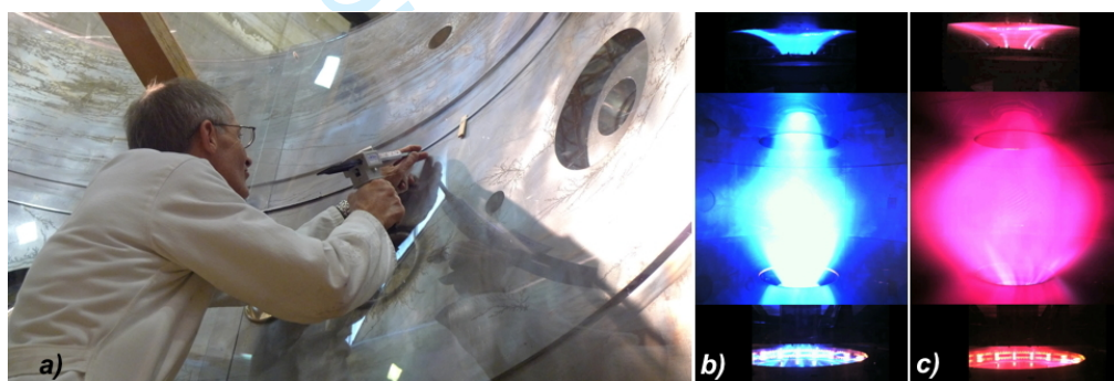
FIGURE 12. (a) Upper diaphragm being glued to the cylindrical large polycarbonate foil with a vacuum compatible strong sealant, able to sustain its weight. (b) Centerpost discharge at full current I_e=10 kA in Argon, shot #954. (c) Centerpost discharge at full current I_e=10 kA in Hydrogen, shot #969.
