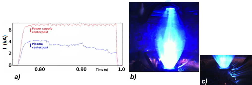
FIGURE 9. (a) Waveforms of Argon centerpost plasma current, evidencing a slow decrease of plasma centerpost current I_c . (b) and (c) Spurious plasma currents with filamentary patterns near the lower PF2 mirror coil. All figures refer to shot #597.
