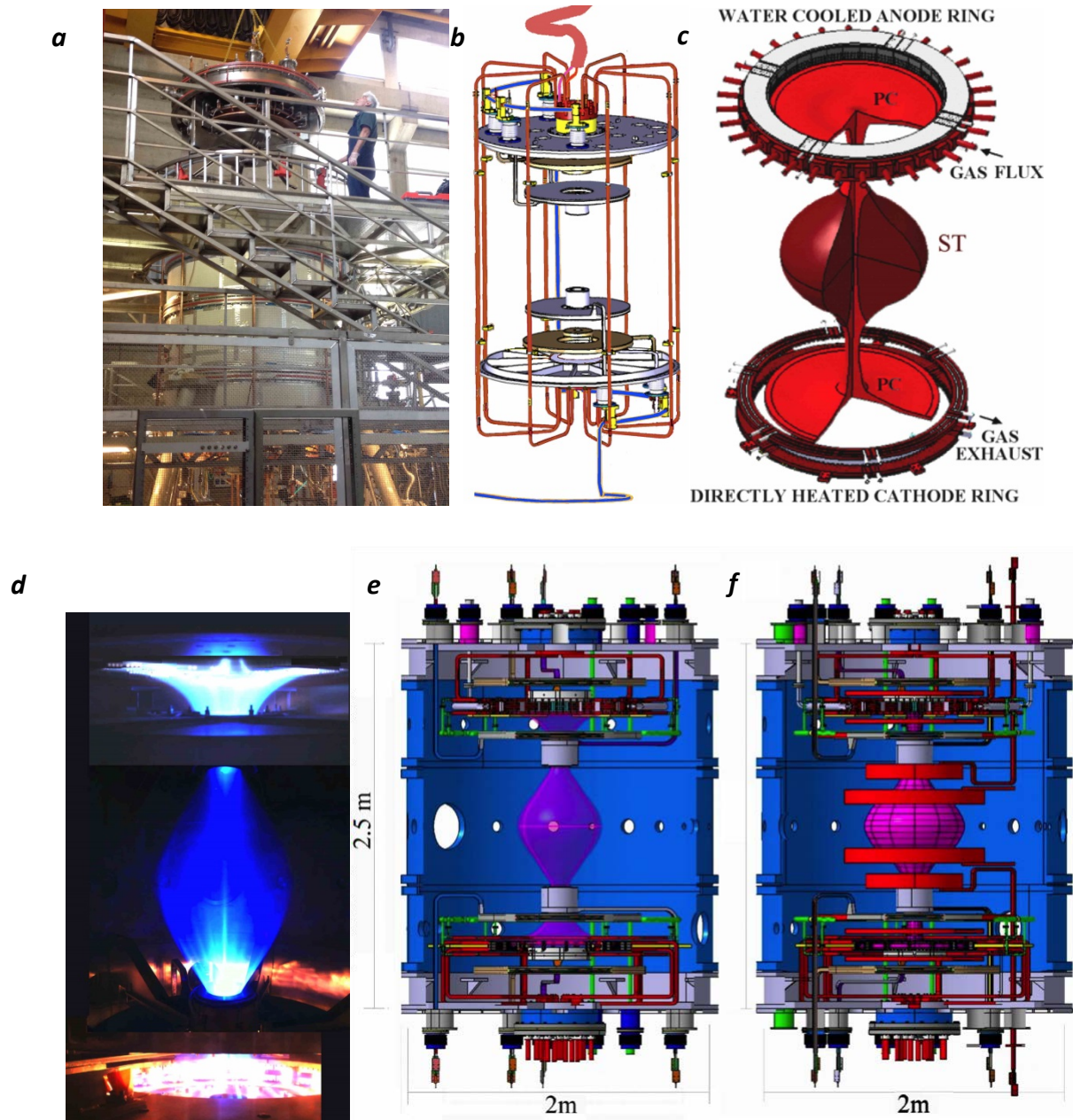
Fig.1: The general layout of the experiment.
