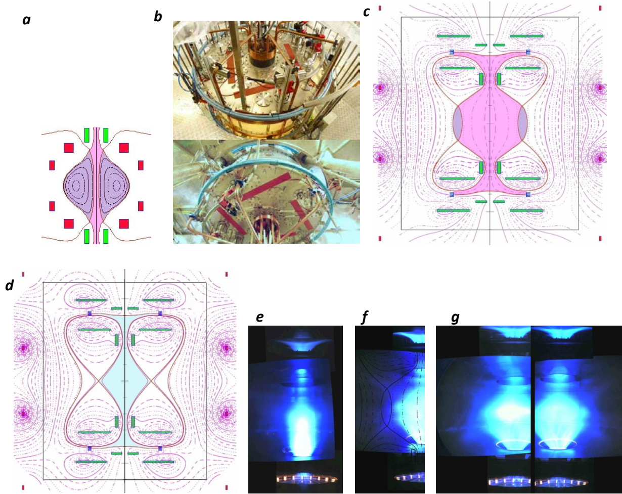
Fig.4: Plasma tori, foreseen for Phase-2 and obtained in Phase-1.
