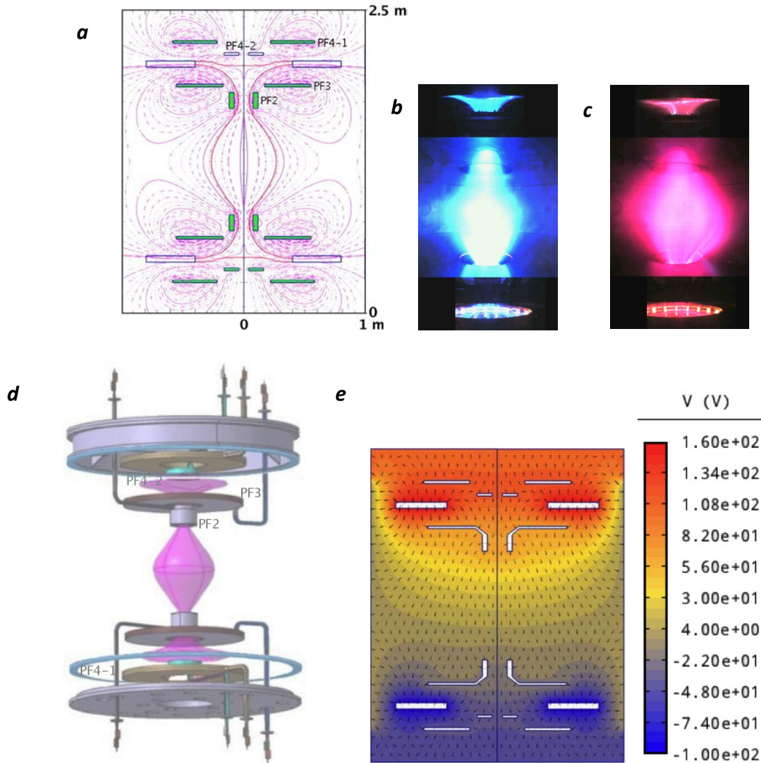
Fig.3: The Plasma-Centerpost produced in Phase-1.
