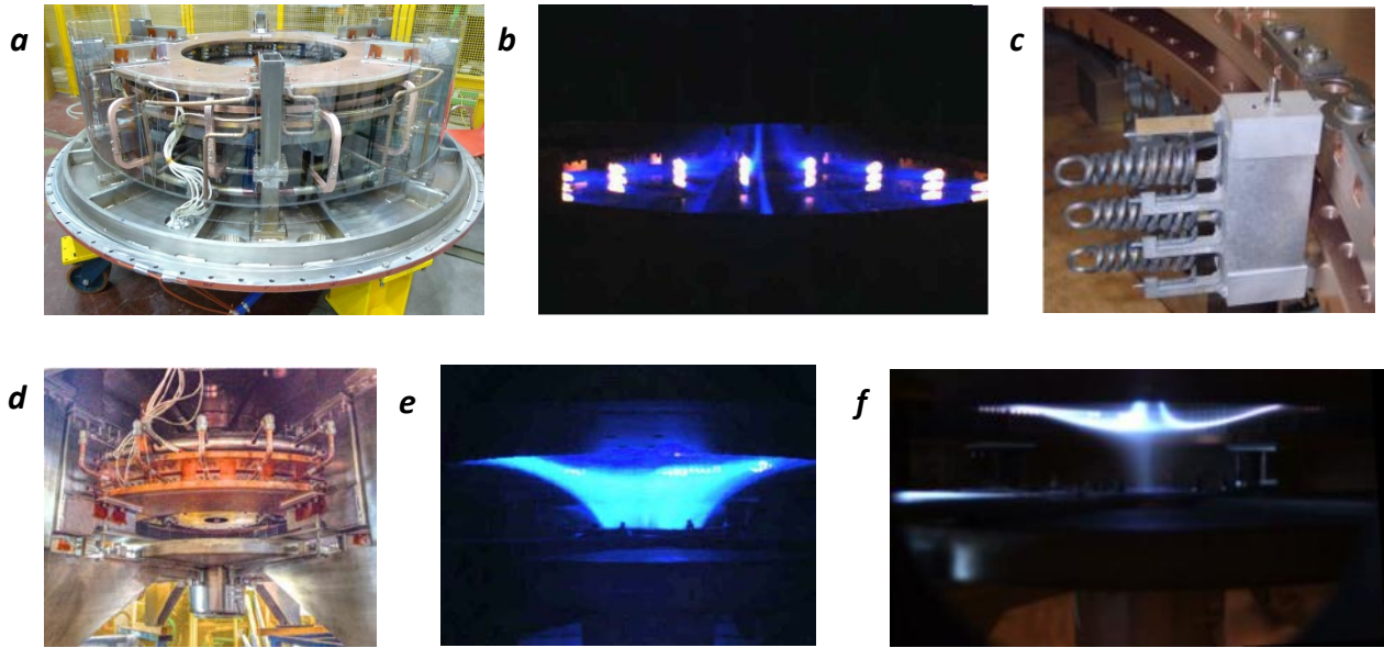
Fig.2: The cathode and the anode of PROTO-SPHERA.
