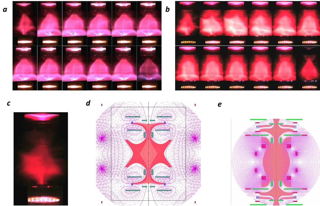
Fig.6: Torus sustained ¼ sec & metamorphosis of a toroidal cusp into a torus.
