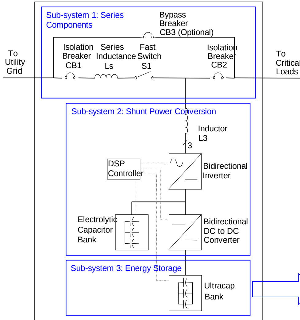
EnergyBridge™ UPS - One-line Diagram
