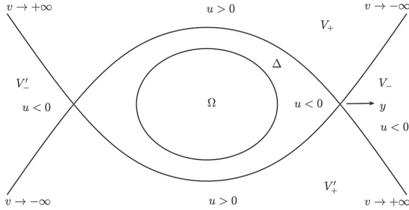
Figure 1. Equilibrium magnetic structure. Note that the y-axis has been rotated by 90^\circ .
