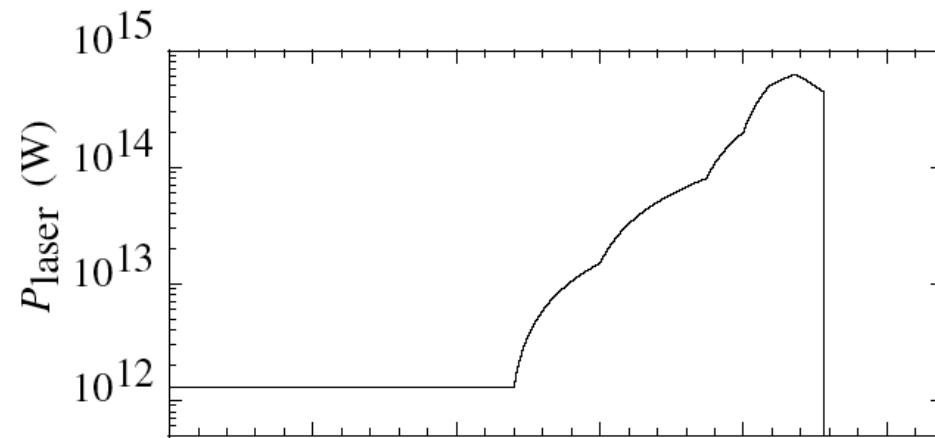
Laser power vs time (notice the log scale)
