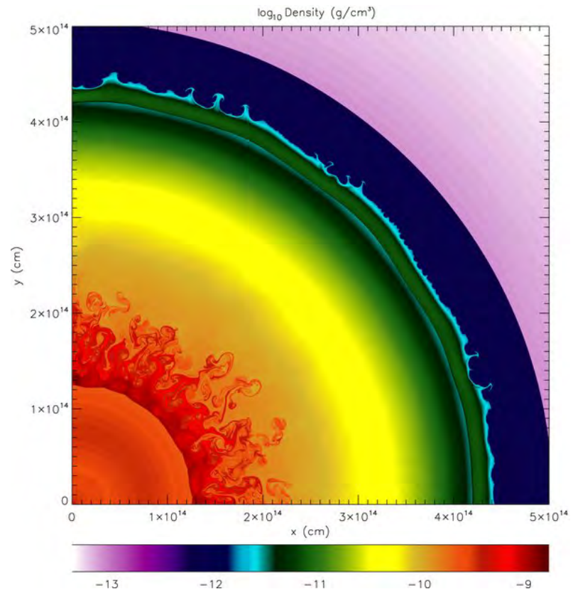
C. C. Joggerst et al., Astroph. J. 693 , 1780 (2009) frame size: 5 \times 10^9 km
