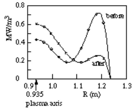
Fig. 2 Radial distribution of the radiated power before and after titanisation.
