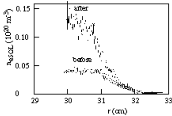
Fig. 3 Experimental profile of electron density in the SOL as a function of the minor radius before and after titanisation
