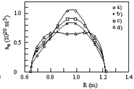
Fig. 4 Time evolution of the electron density profile starting from: a) before titanisation, b) just after titanisation, c) after 8 shots, d) after 11 shots when Ti film is fully H-saturated
