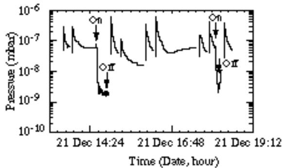
Fig. 1. Temporal evolution of pressure inside the machine during the time interval between pulses.
